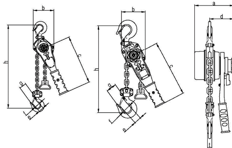
PLH080WO/ PLH100WO
