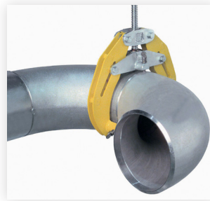
Fit up two 90° fittings
