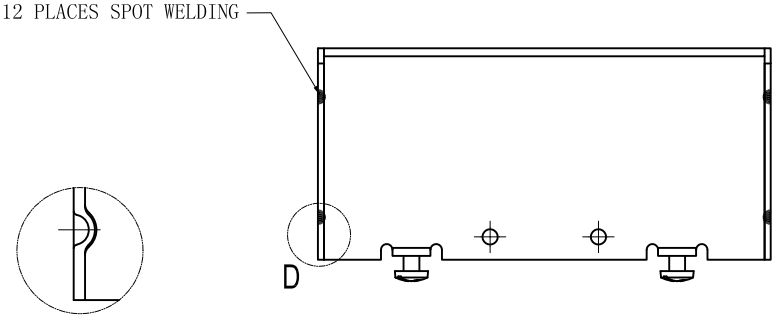
WELDING STYLE DETAIL VIEW D
