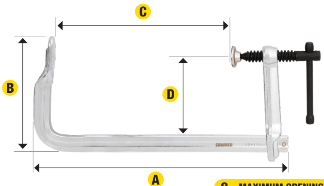
C = MAXIMUM OPENING
