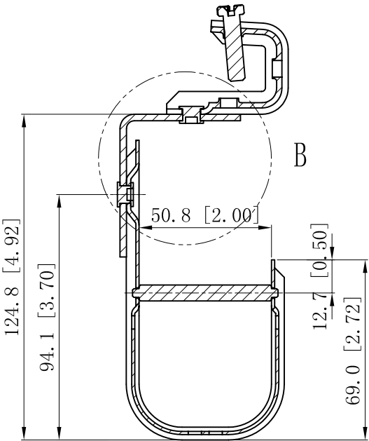
CUTAWAY VIEW A-A
