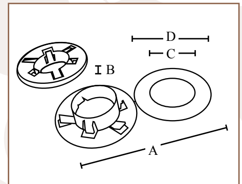
Common hole configurations in metal studs
