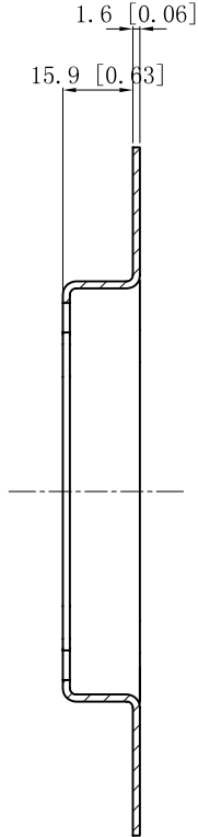
CUTAWAY VIEW A-A
