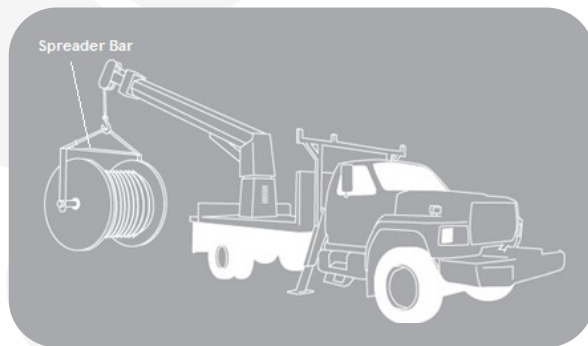
Figure 2: Crane handling of reels.
