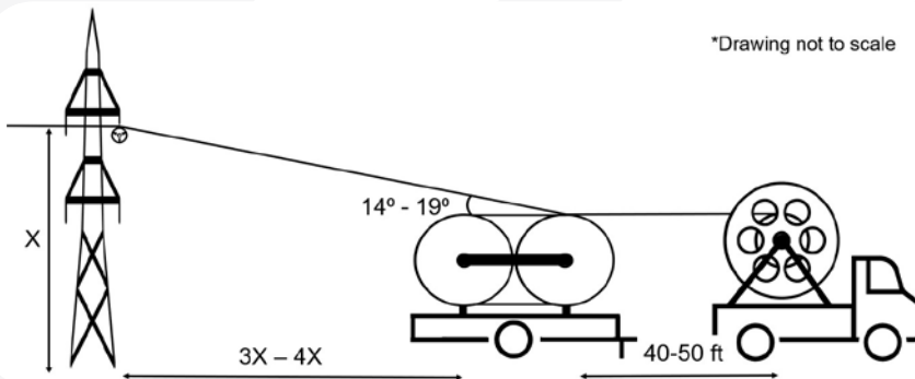
Figure 10: Orientation for bullsheel/payoff setup.
