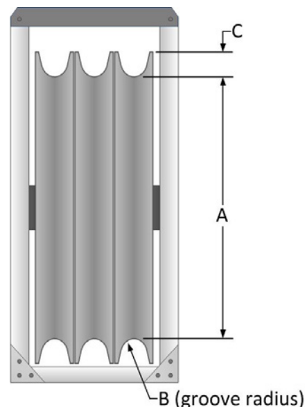
Figure 11: Measurements for stringing sheave.
