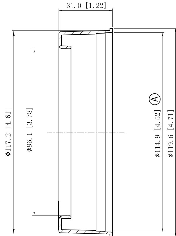
CUTAWAY VIEW A-A
