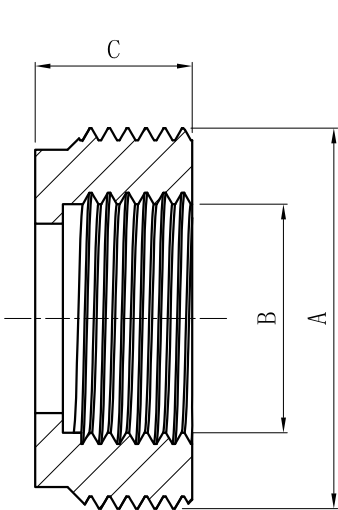
CUTAWAY VIEW A-A
