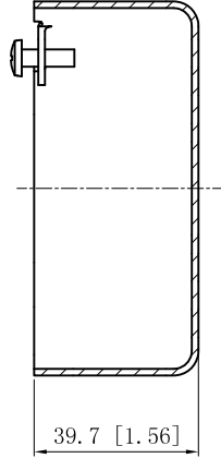
CUTAWAY VIEW A-A
