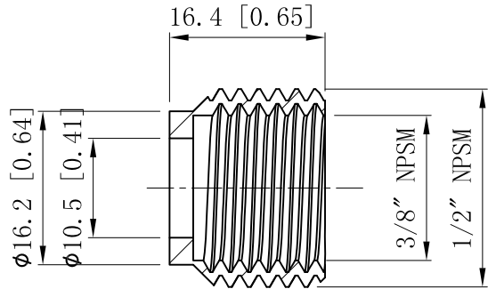
CUTAWAY VIEW A-A
